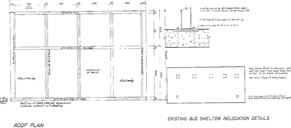
ROOF PLAN
