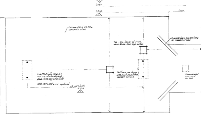
SLAB PLAN
