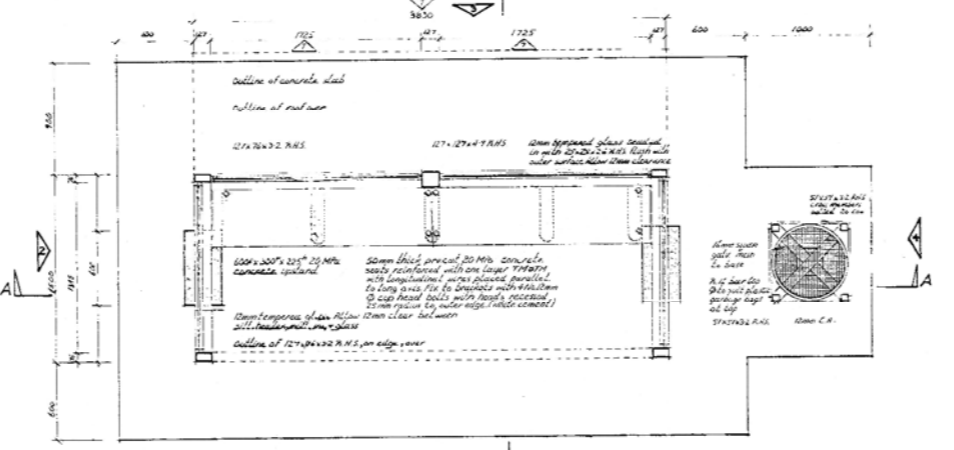
PLAN (Glazing level)
