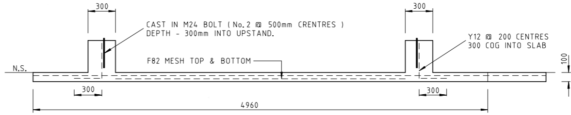
SLAB DETAILS - SECTION "A - A"
