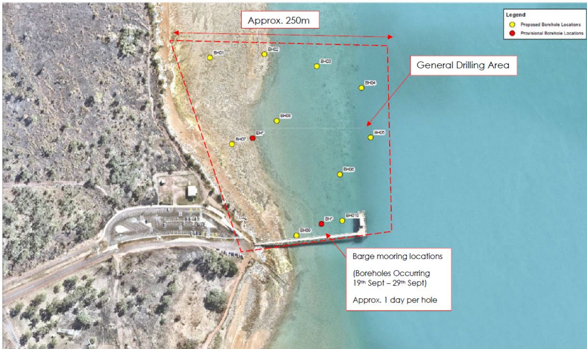
Figure 2: Extent of works around the Jetty.
