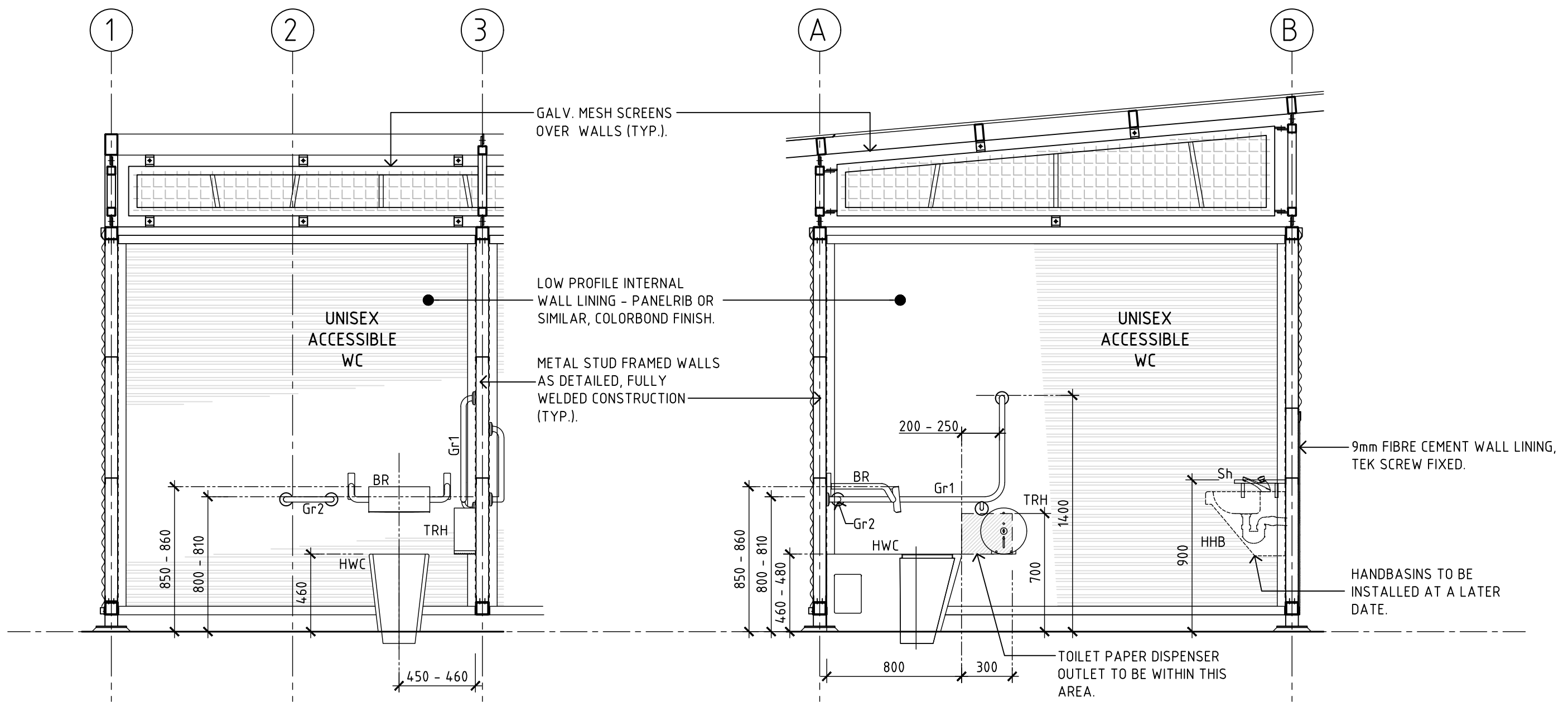
5 ELEVATION A01 SCALE - 1:25
