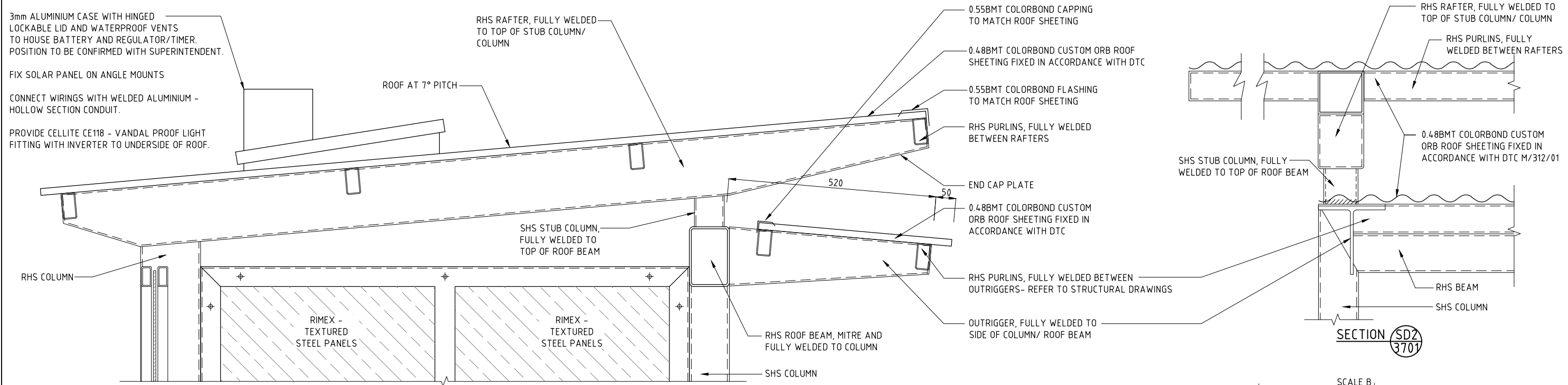
SECTION SD1 SCALE B
