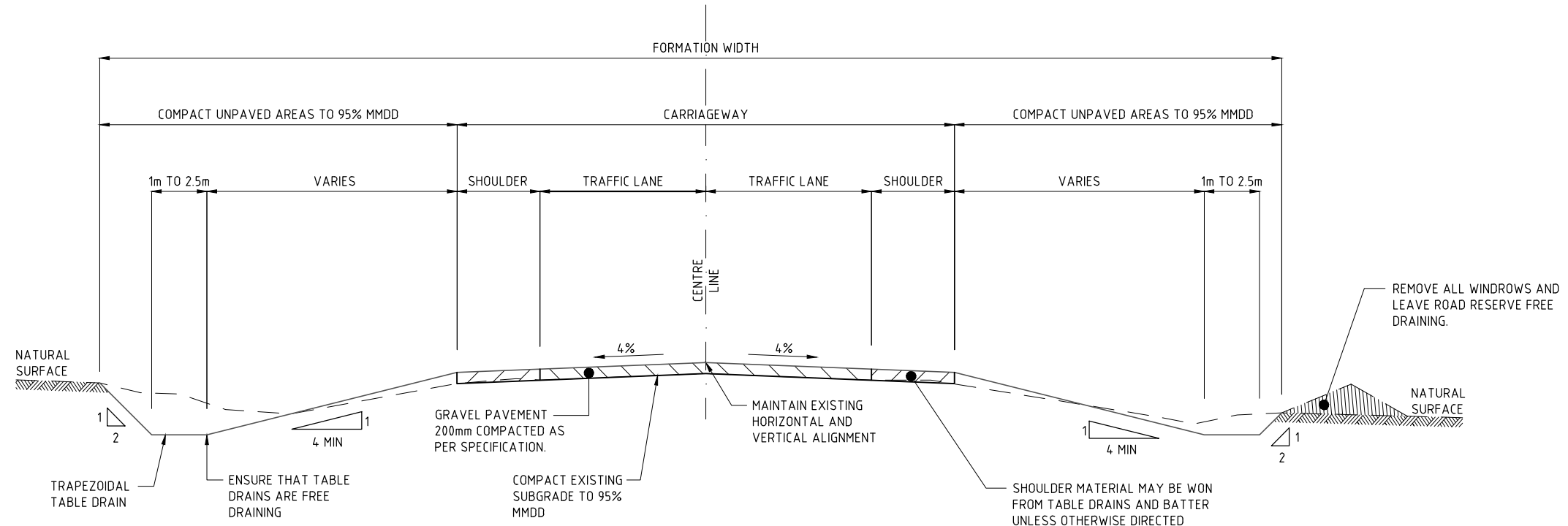
TYPICAL CROSS SECTION GRAVEL ROADS REFER TO TABLE FOR TRAFFIC LANE, SHOULDER AND CARRIAGEWAY WIDTHS.
