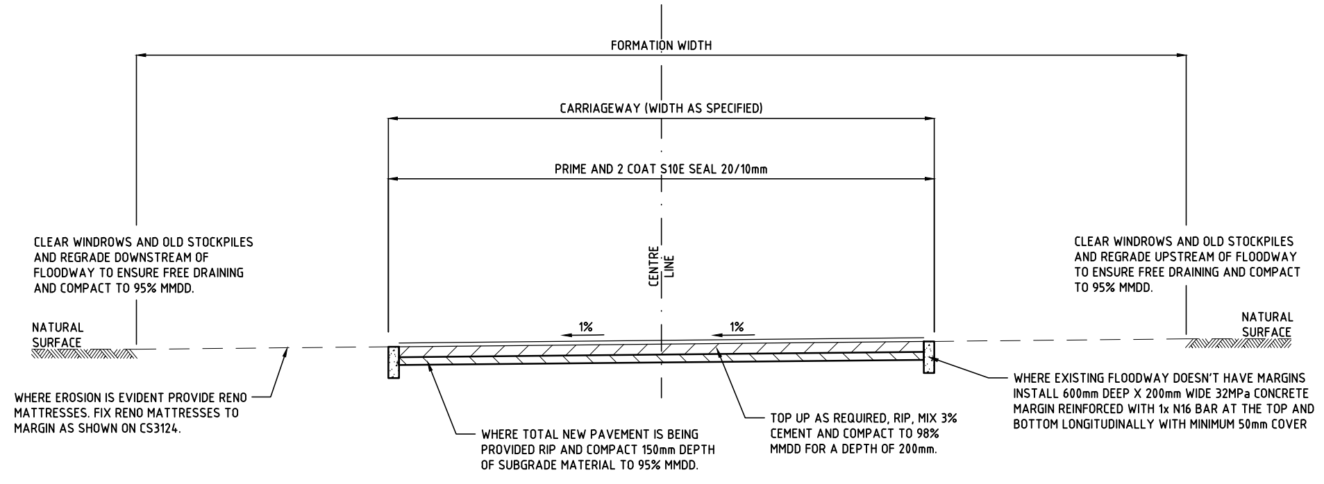
TYPICAL FLOODWAY CROSS SECTION
