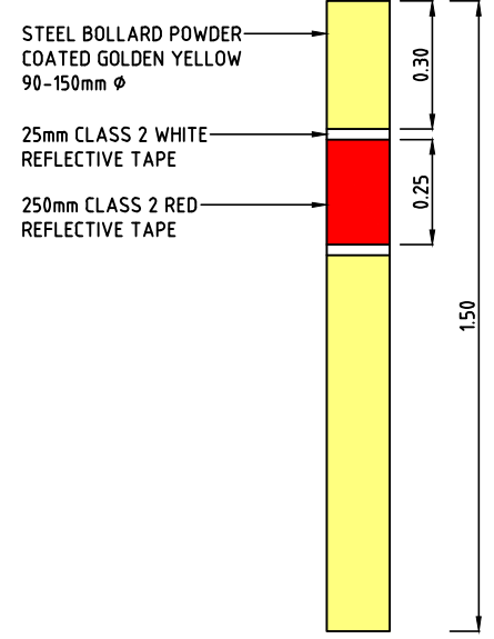
TYPICAL BOLLARD
