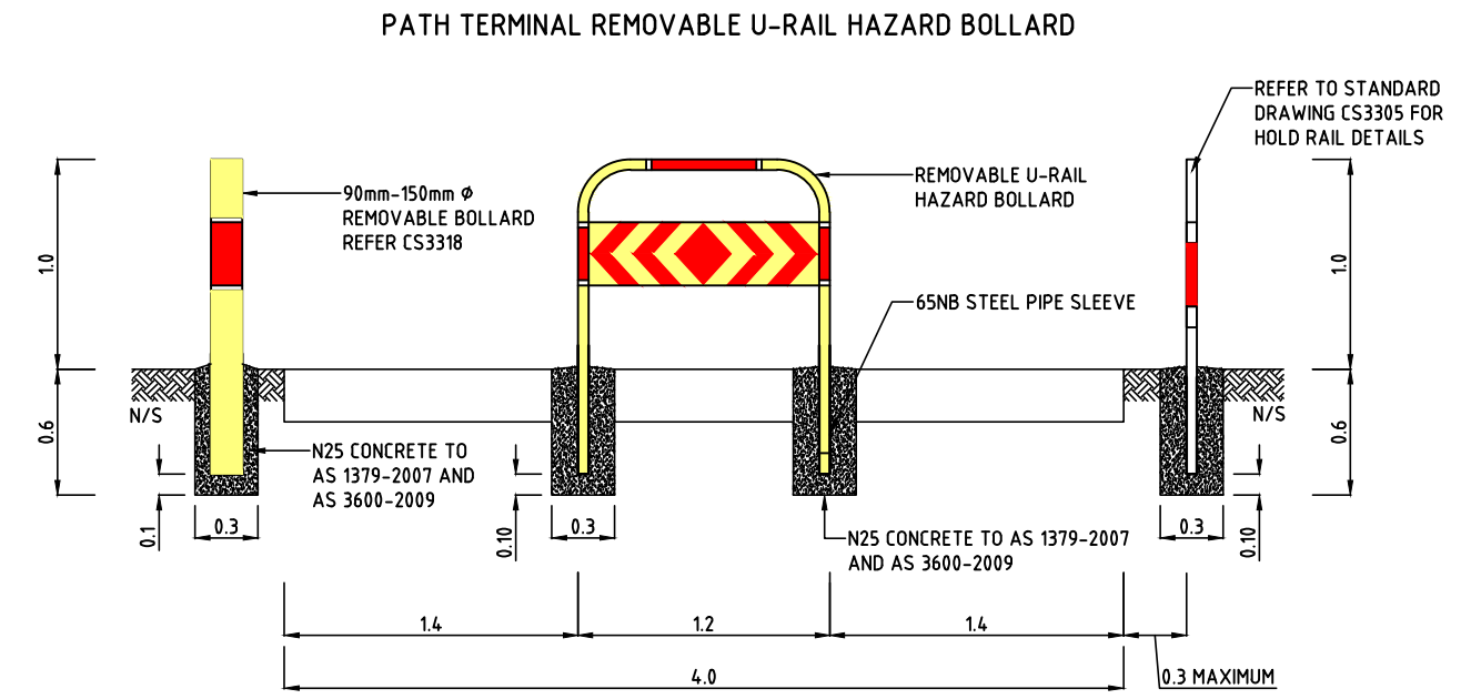
TYPICAL SECTION
